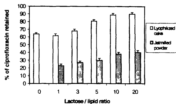
Figure 1. Histogram representation of ciprofloxacin retention (%) of reconstituted liposomes as a function of lactose concentration ( n = 3 , error bars indicate SD).
