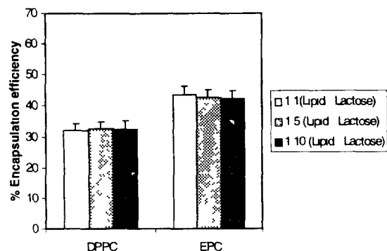
Figure 2. Histogram representation of percent encapsulation efficiency of ciprofloxacin (in spontaneously formed liposomes) on dispersion of DPPC- and EPC-based formulations at various concentrations of lactose (lipid concentration, 0.1 M; n = 3 ; error bars indicate SD)
